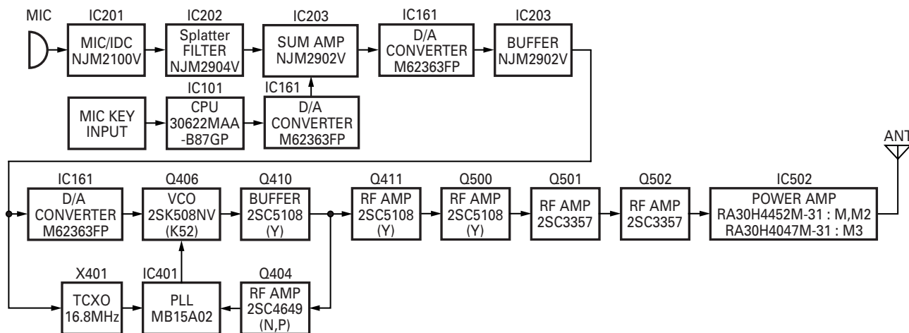
Fig. 8 Transmitter system
